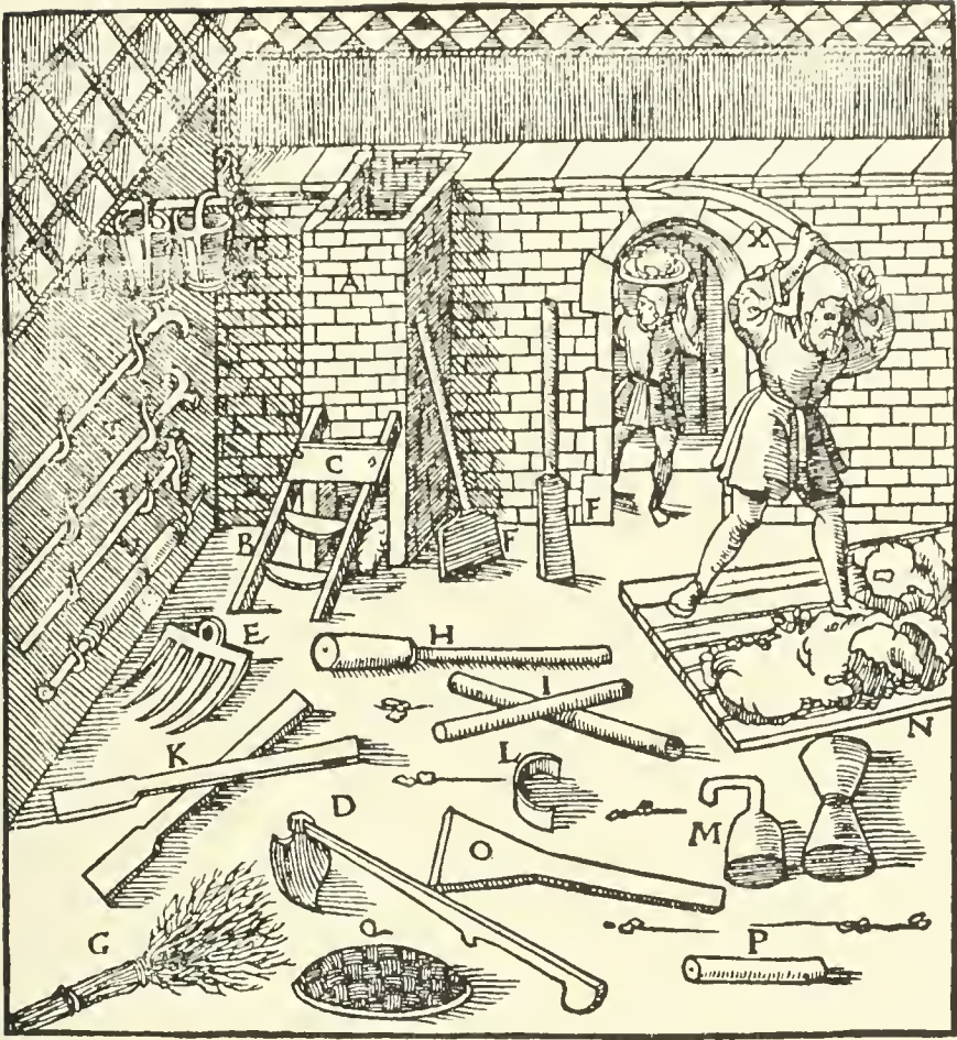
A—FURNACE. B—LADDER. C—BOARD FIXED TO IT. D—HOE. E—FIVE-TOOTHED RAKE. F—WOODEN SPATULA. G—BROOM. H—RAMMER. I—RAMMER, SAME DIAMETER. K—TWO WOODEN SPATULAS. L—CURVED BLADE. M—BRONZE RAMMER. N—ANOTHER BRONZE RAMMER. O—WIDE SPATULA. P—ROD. Q—WICKER BASKET. R—TWO BUCKETS OF LEATHER IN WHICH WATER IS CARRIED FOR PUTTING OUT A CONFLAGRATION, SHOULD THE officina CATCH FIRE. S—BRASS PUMP WITH WHICH THE WATER IS SQUIRTED OUT. T—TWO HOOKS. V—RAKE. X—WORKMAN BEATING THE CLAY WITH AN IRON IMPLEMENT.
